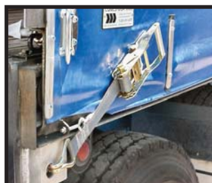
Ratchet Assemblies
